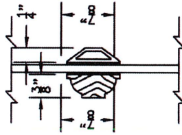
7/8" SQUARE SIMULATED DIVIDED LITE SINGLE GLAZED GLASS
